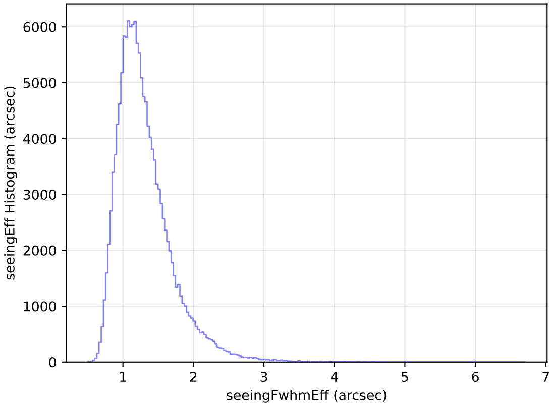
internal_u_expt38_nscale1.2v3.4_10yrs WFD u band: seeingEff Histogram
