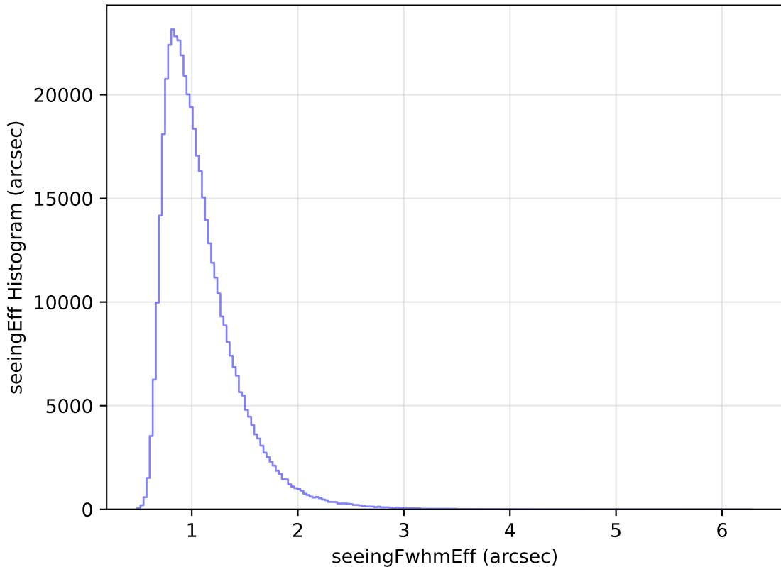
internal_u_expt38_nscale1.2v3.4_10yrs WFD i band: seeingEff Histogram
