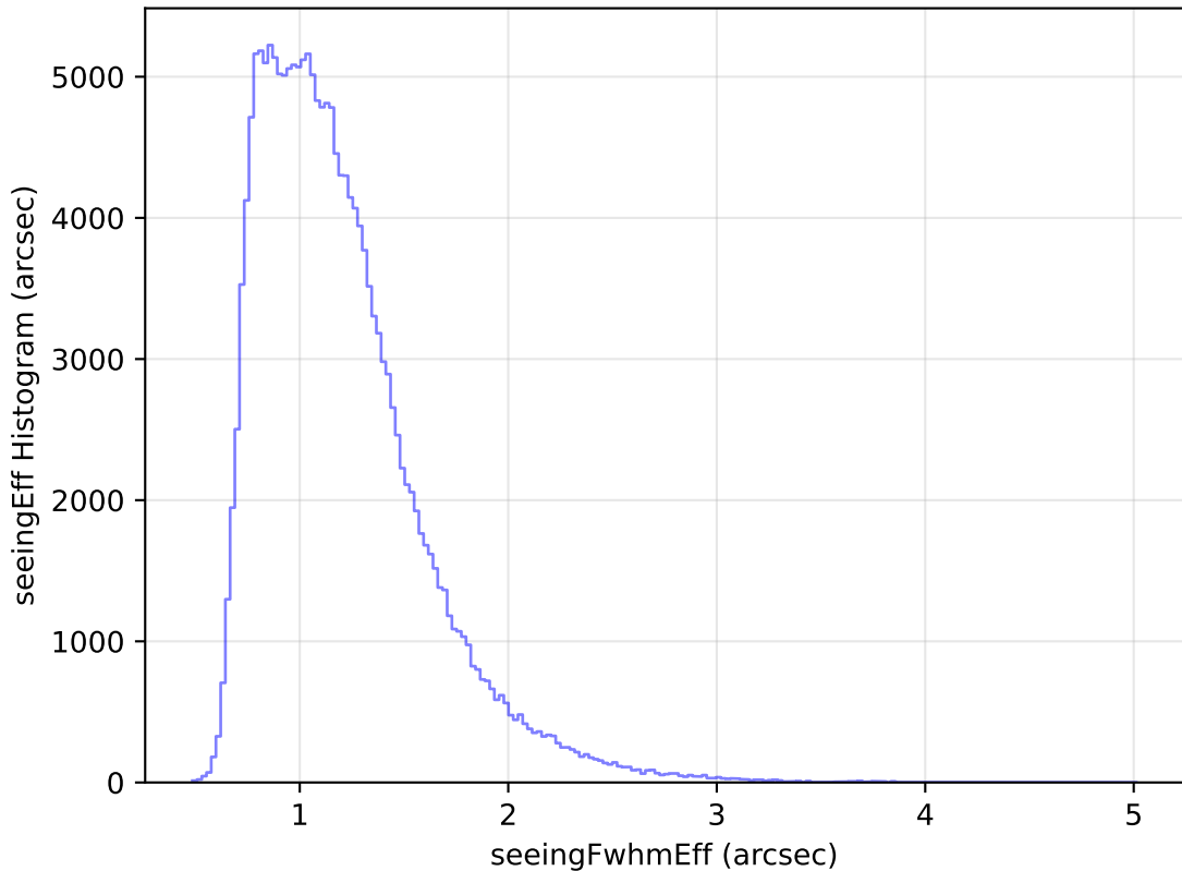
internal_u_expt38_nscale1.2v3.4_10yrs WFD g band: seeingEff Histogram
