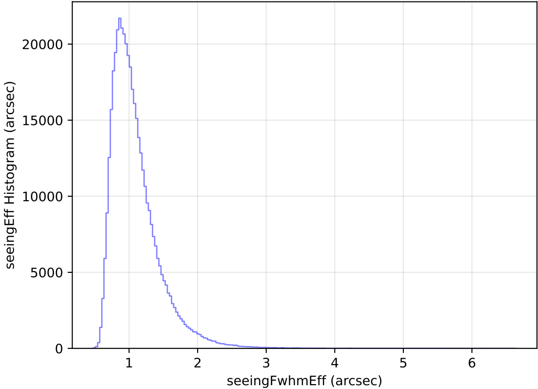
internal_u_expt38_nscale1.2v3.4_10yrs All sky z band: seeingEff Histogram
