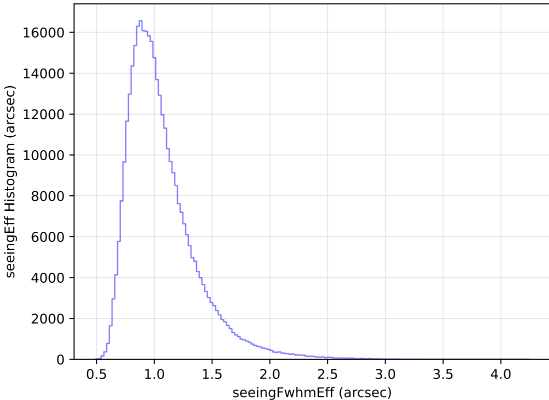
internal_u_expt38_nscale1.2v3.4_10yrs All sky y band: seeingEff Histogram
