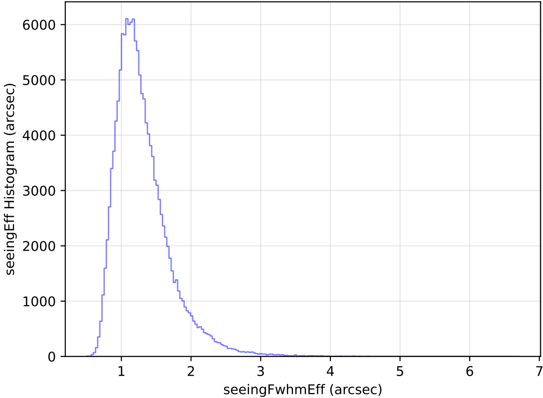
internal_u_expt38_nscale1.2v3.4_10yrs All sky u band: seeingEff Histogram
