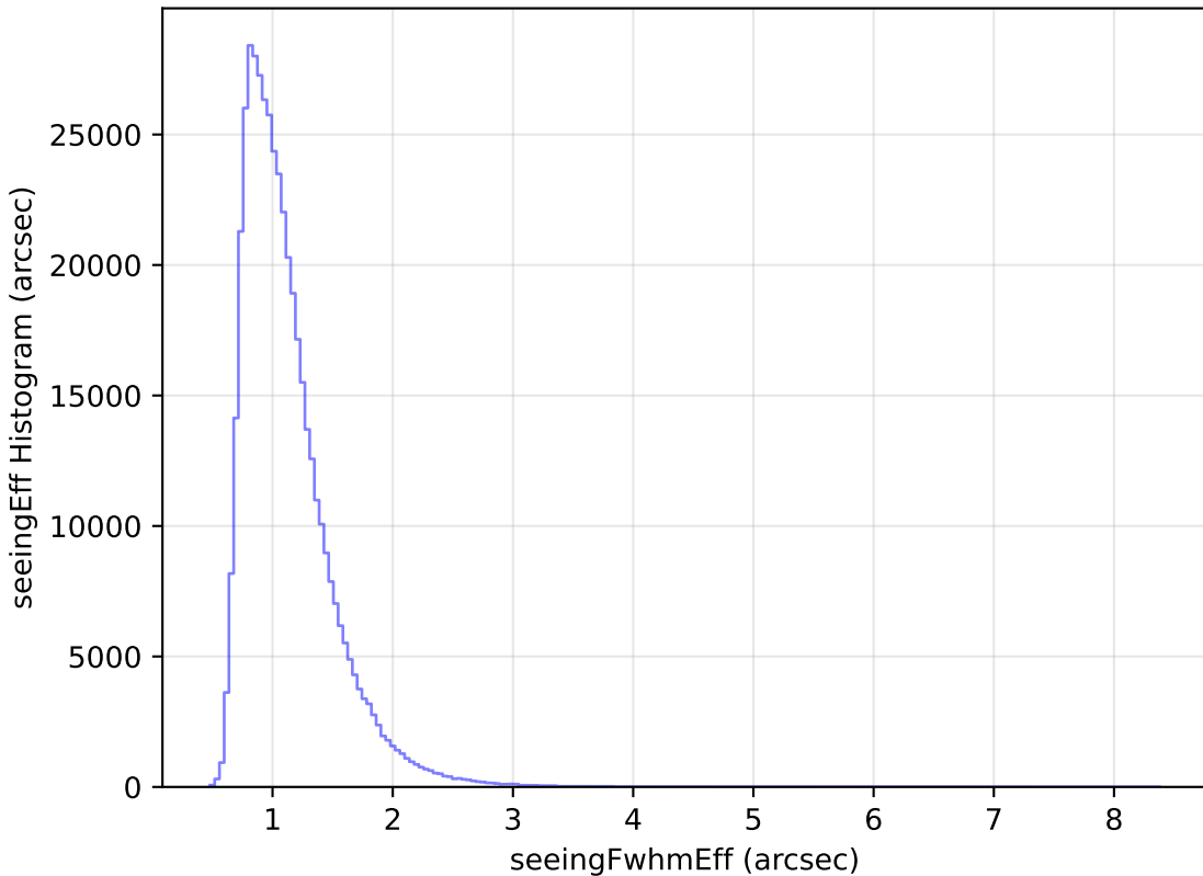
internal_u_expt38_nscale1.2v3.4_10yrs All sky r band: seeingEff Histogram
