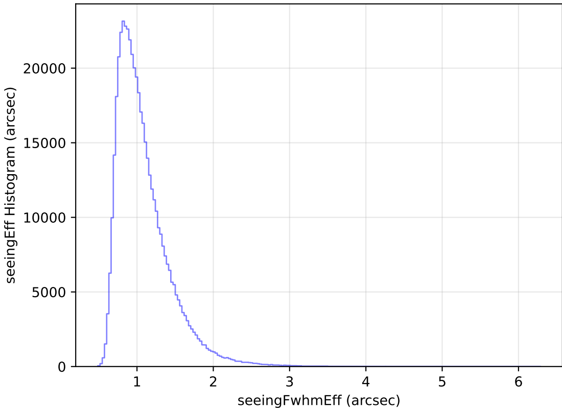
internal_u_expt38_nscale1.2v3.4_10yrs All sky i band: seeingEff Histogram
