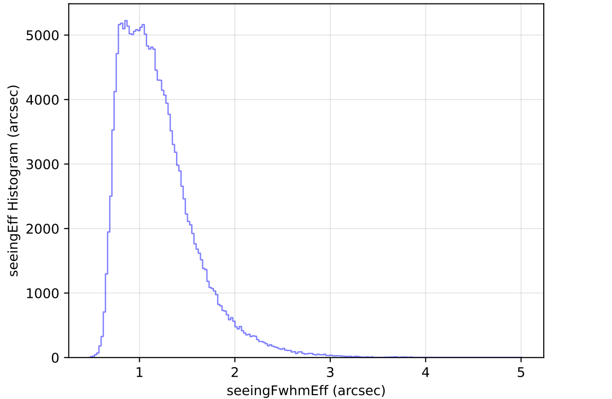
internal_u_expt38_nscale1.2v3.4_10yrs All sky g band: seeingEff Histogram
