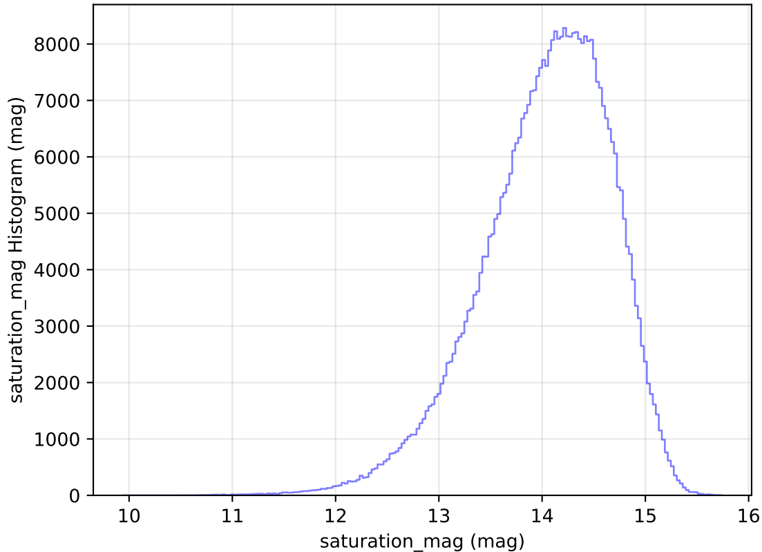
internal_u_expt38_nscale1.2v3.4_10yrs WFD z band: saturation_mag Histogram
