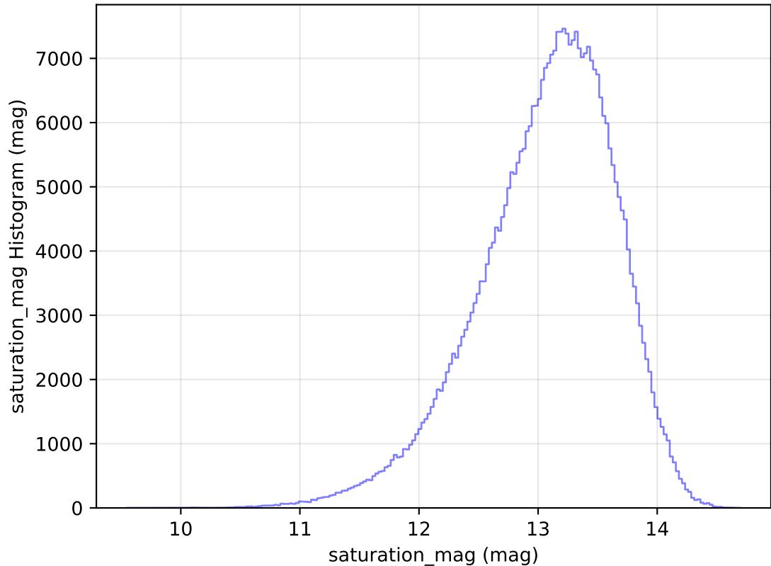
internal_u_expt38_nscale1.2v3.4_10yrs WFD y band: saturation_mag Histogram
