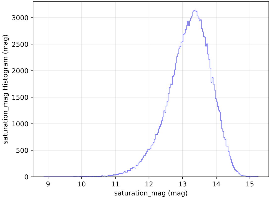
internal_u_expt38_nscale1.2v3.4_10yrs WFD u band: saturation_mag Histogram
