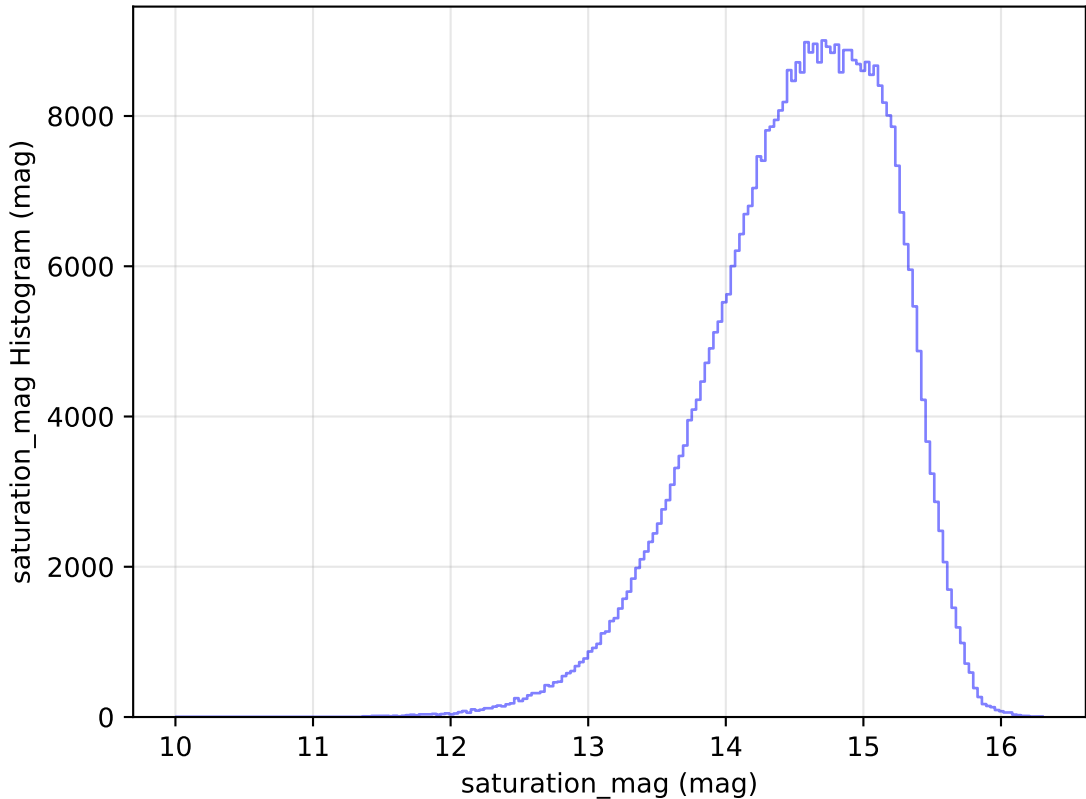
internal_u_expt38_nscale1.2v3.4_10yrs WFD r band: saturation_mag Histogram
