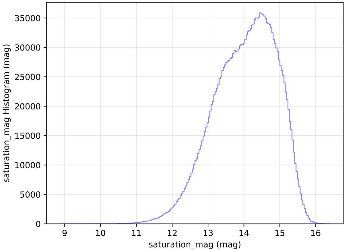
internal_u_expt38_nscale1.2v3.4_10yrs WFD all bands: saturation_mag Histogram
