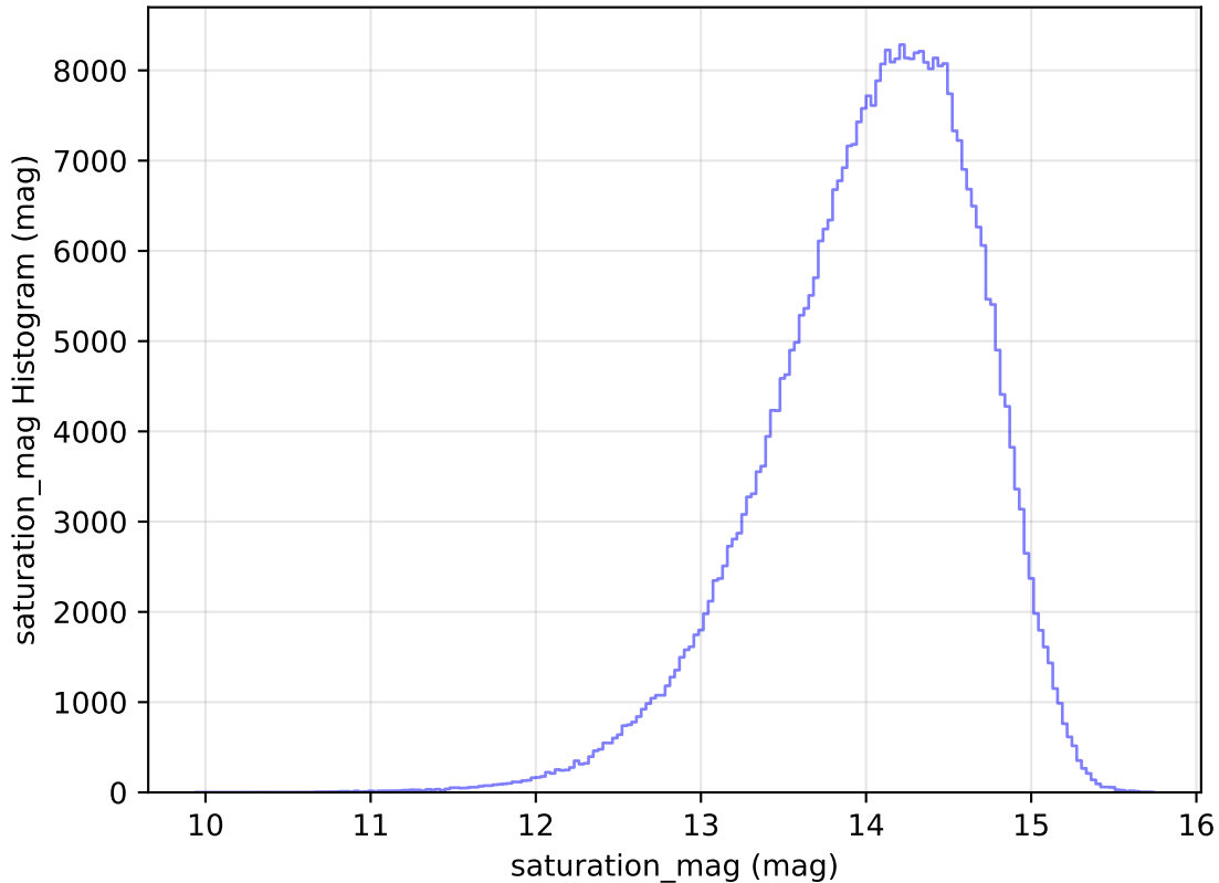
internal_u_expt38_nscale1.2v3.4_10yrs All sky z band: saturation_mag Histogram
