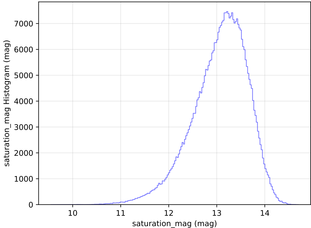
internal_u_expt38_nscale1.2v3.4_10yrs All sky y band: saturation_mag Histogram
