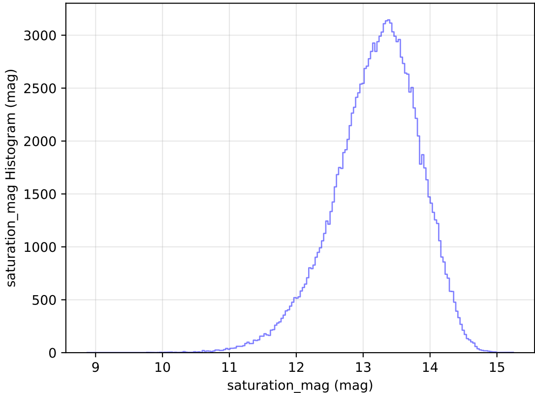
internal_u_expt38_nscale1.2v3.4_10yrs All sky u band: saturation_mag Histogram
