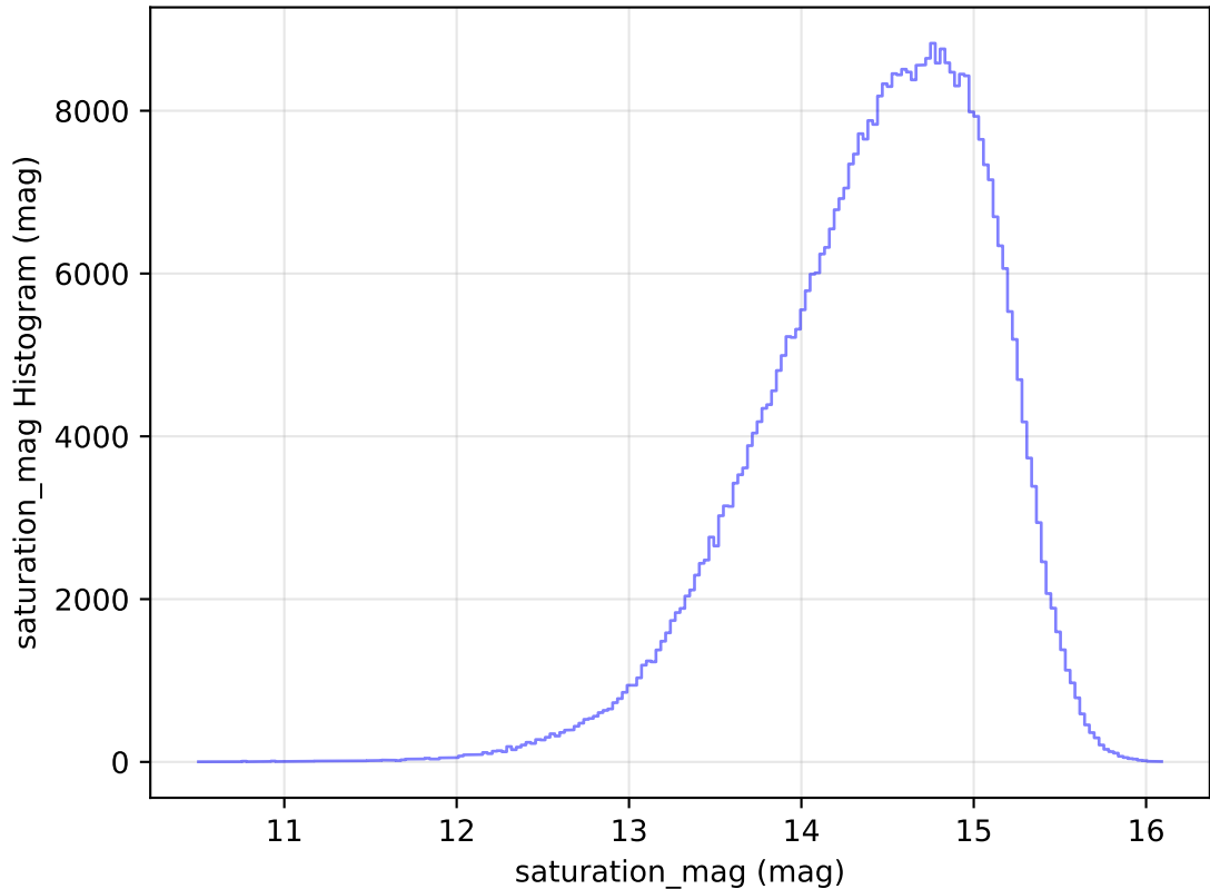
internal_u_expt38_nscale1.2v3.4_10yrs All sky i band: saturation_mag Histogram
