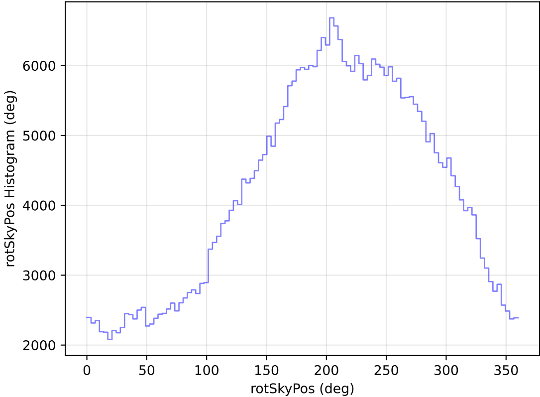
internal_u_expt38_nscale1.2v3.4_10yrs WFD z band: rotSkyPos Histogram
