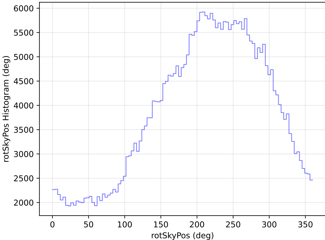
internal_u_expt38_nscale1.2v3.4_10yrs WFD y band: rotSkyPos Histogram
