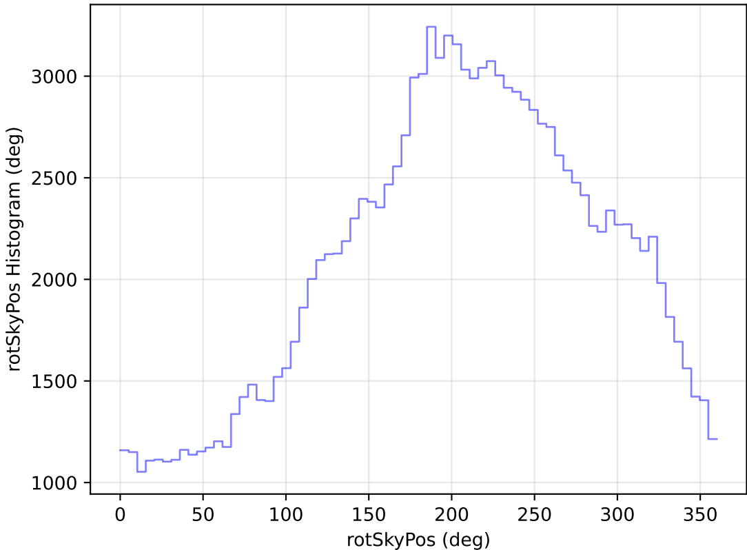
internal_u_expt38_nscale1.2v3.4_10yrs WFD u band: rotSkyPos Histogram
