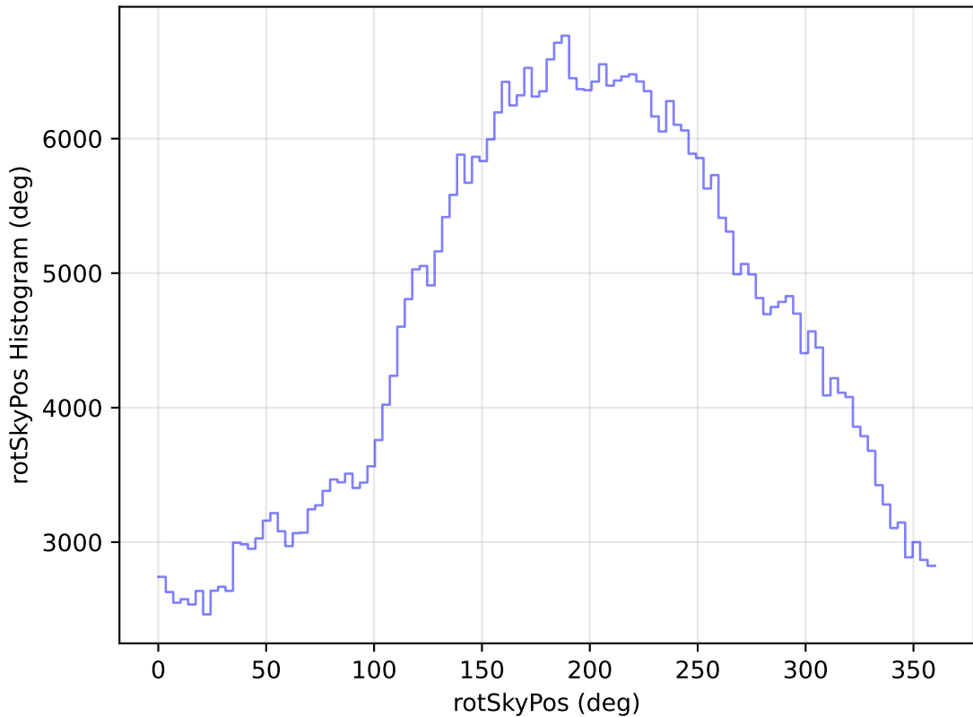
internal_u_expt38_nscale1.2v3.4_10yrs WFD r band: rotSkyPos Histogram
