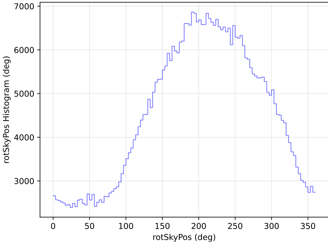
internal_u_expt38_nscale1.2v3.4_10yrs WFD i band: rotSkyPos Histogram
