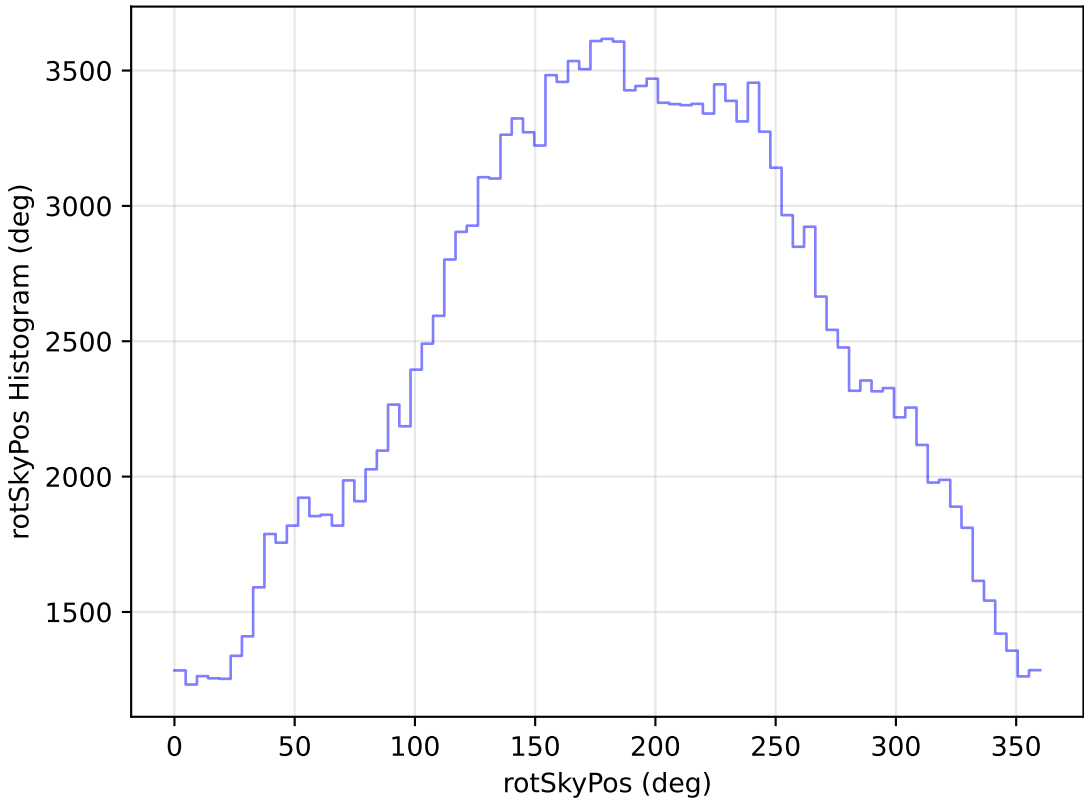
internal_u_expt38_nscale1.2v3.4_10yrs WFD g band: rotSkyPos Histogram
