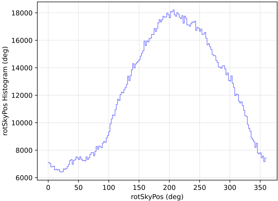
internal_u_expt38_nscale1.2v3.4_10yrs WFD all bands: rotSkyPos Histogram
