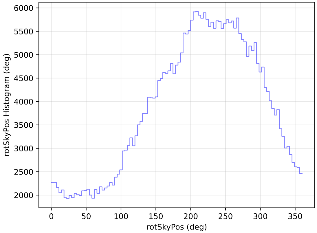
internal_u_expt38_nscale1.2v3.4_10yrs All sky y band: rotSkyPos Histogram
