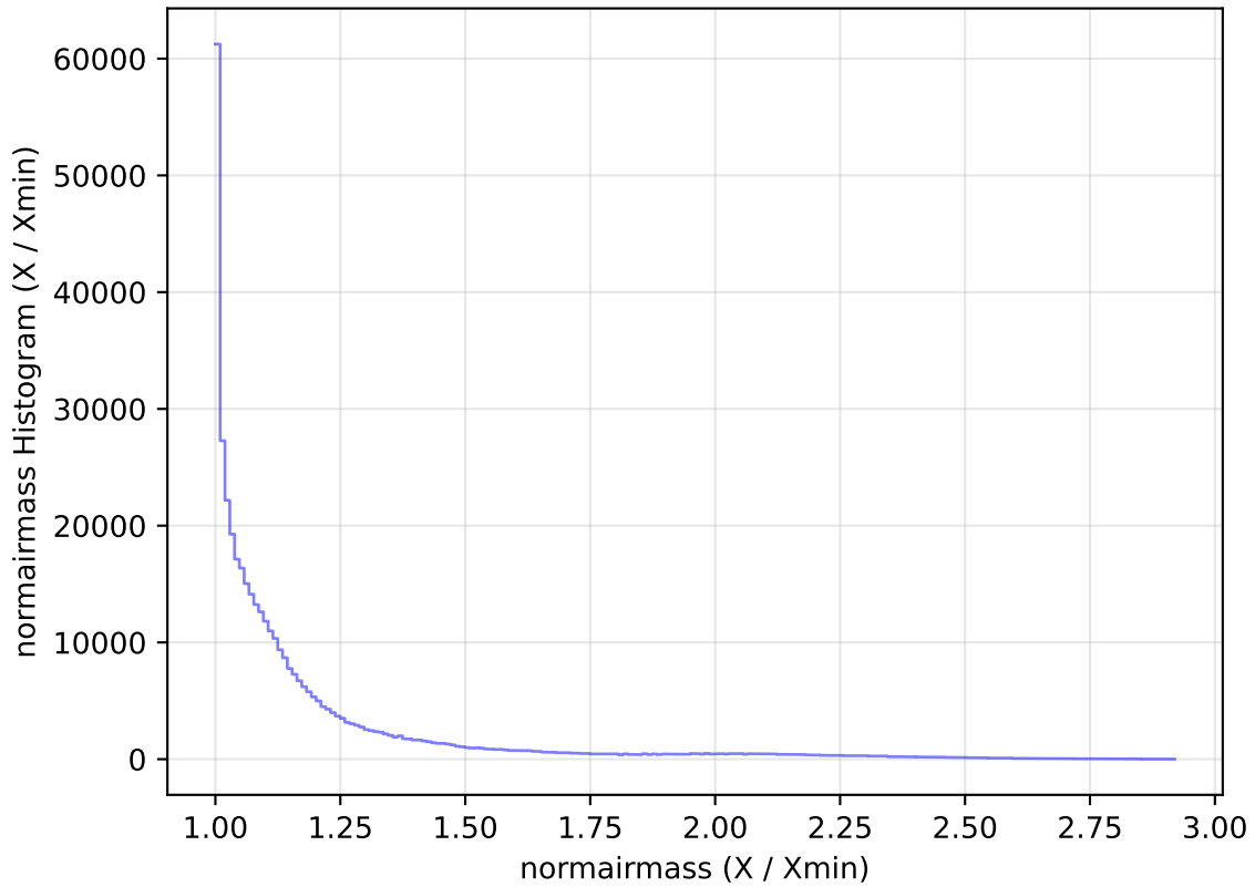
internal_u_expt38_nscale1.2v3.4_10yrs WFD z band: normairmass Histogram
