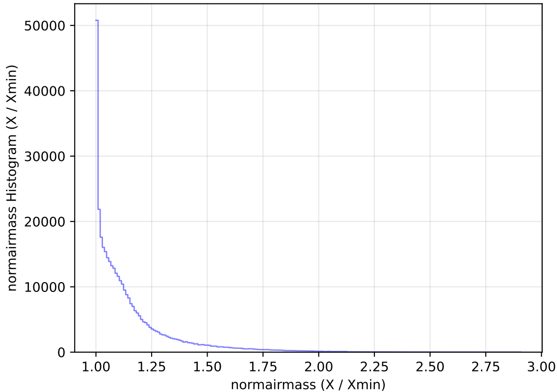
internal_u_expt38_nscale1.2v3.4_10yrs WFD y band: normairmass Histogram
