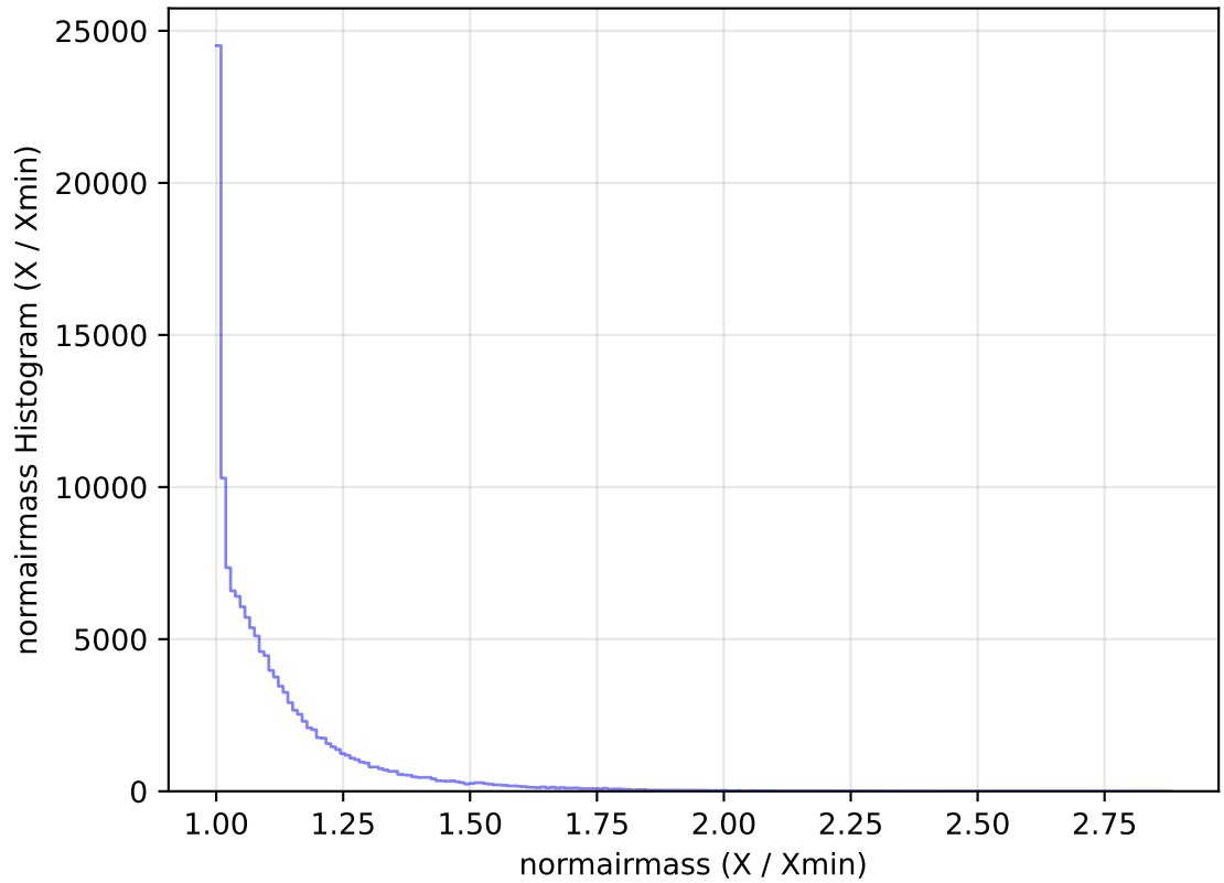
internal_u_expt38_nscale1.2v3.4_10yrs WFD u band: normairmass Histogram
