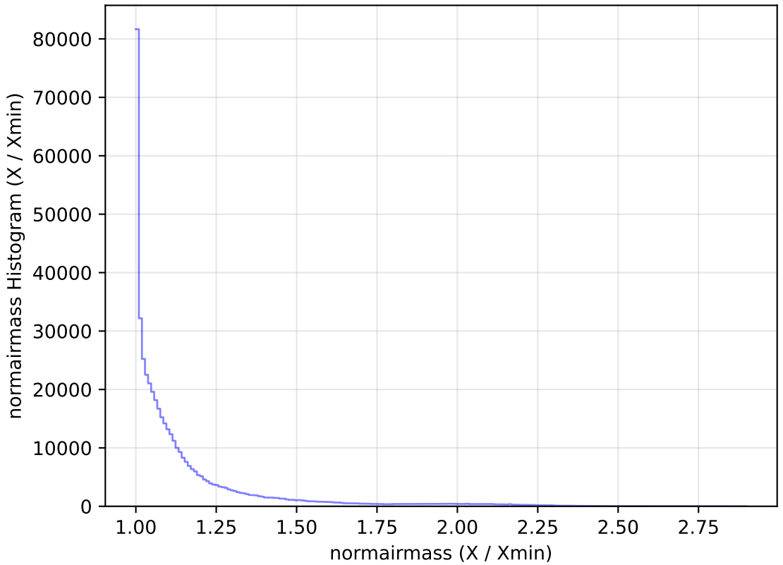
internal_u_expt38_nscale1.2v3.4_10yrs WFD r band: normairmass Histogram
