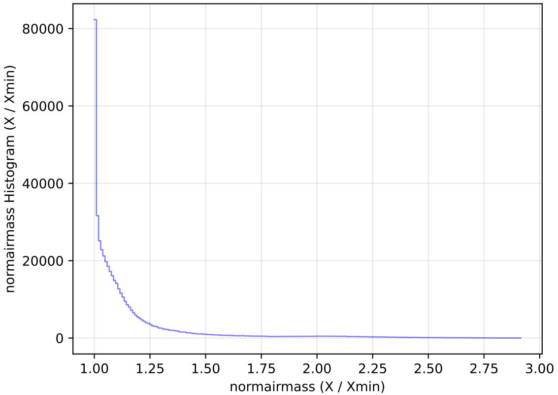
internal_u_expt38_nscale1.2v3.4_10yrs WFD i band: normairmass Histogram
