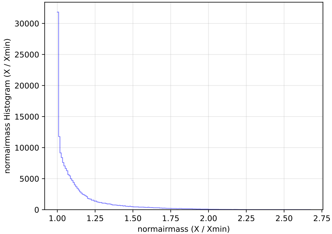
internal_u_expt38_nscale1.2v3.4_10yrs WFD g band: normairmass Histogram
