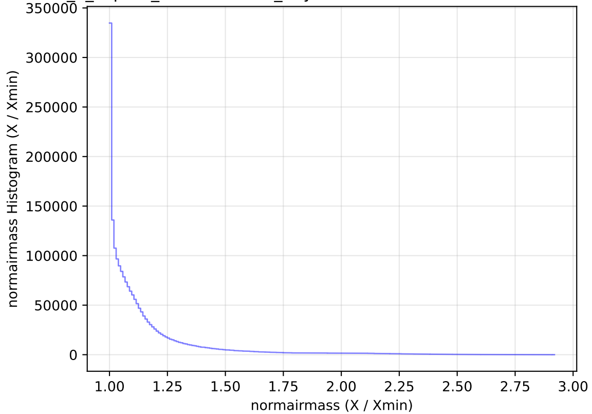
internal_u_expt38_nscale1.2v3.4_10yrs WFD all bands: normairmass Histogram
