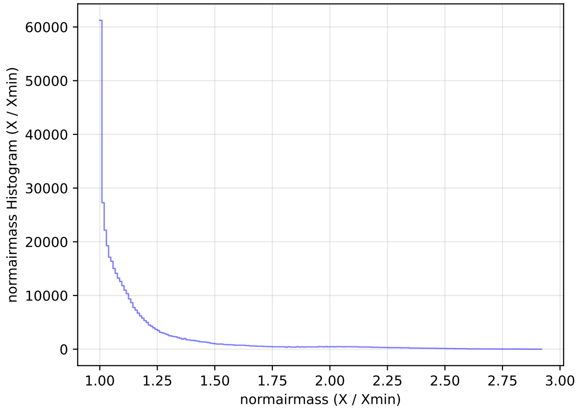
internal_u_expt38_nscale1.2v3.4_10yrs All sky z band: normairmass Histogram
