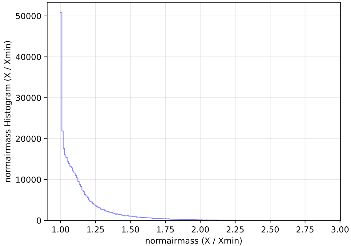
internal_u_expt38_nscale1.2v3.4_10yrs All sky y band: normairmass Histogram
