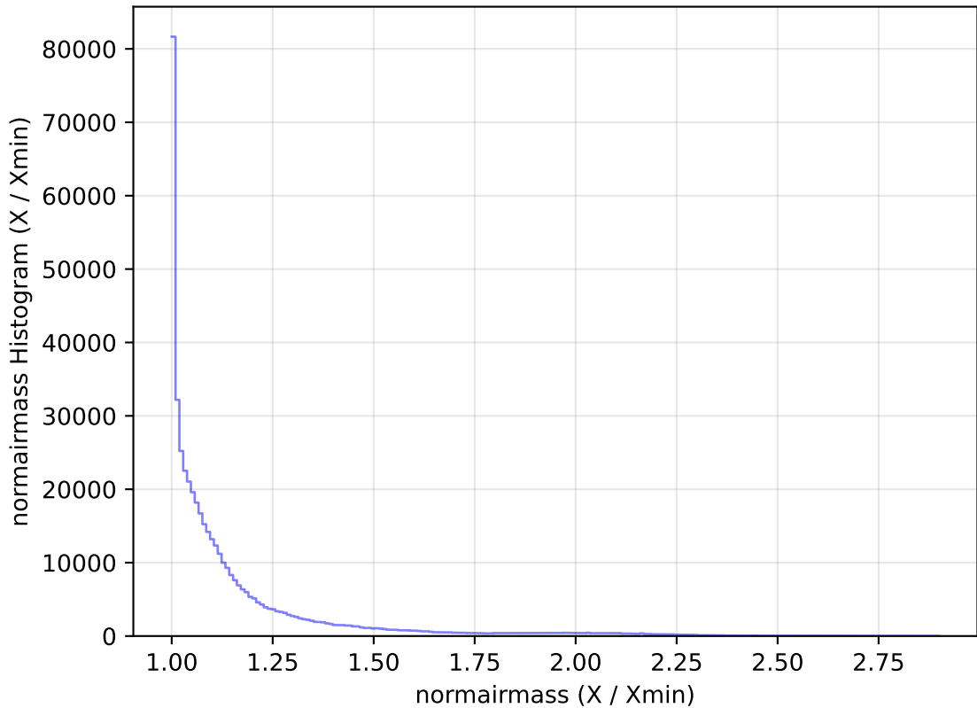
internal_u_expt38_nscale1.2v3.4_10yrs All sky r band: normairmass Histogram
