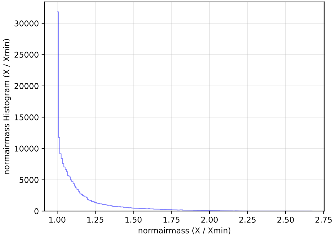
internal_u_expt38_nscale1.2v3.4_10yrs All sky g band: normairmass Histogram
