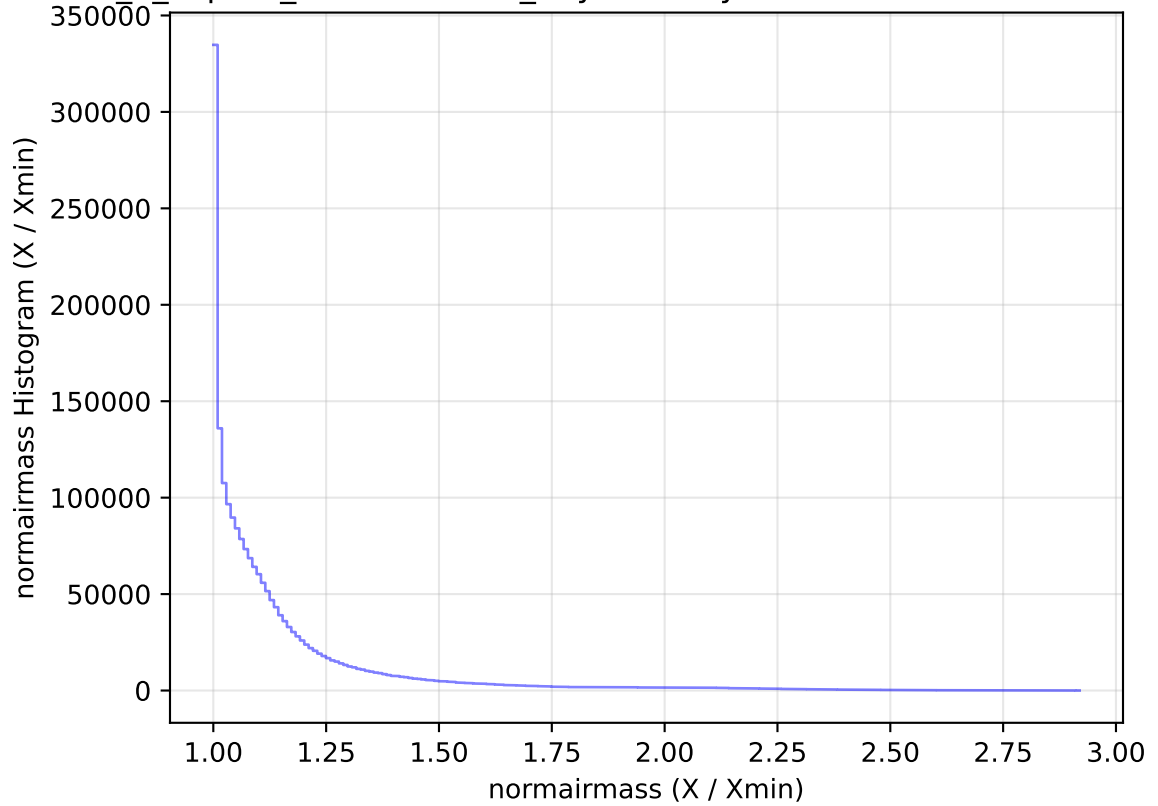
internal_u_expt38_nscale1.2v3.4_10yrs All sky all bands: normairmass Histogram
