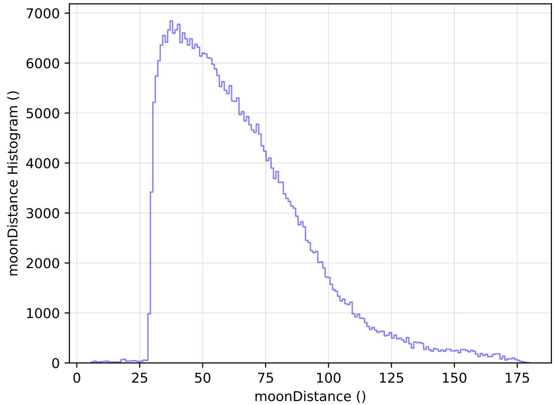
internal_u_expt38_nscale1.2v3.4_10yrs WFD y band: moonDistance Histogram
