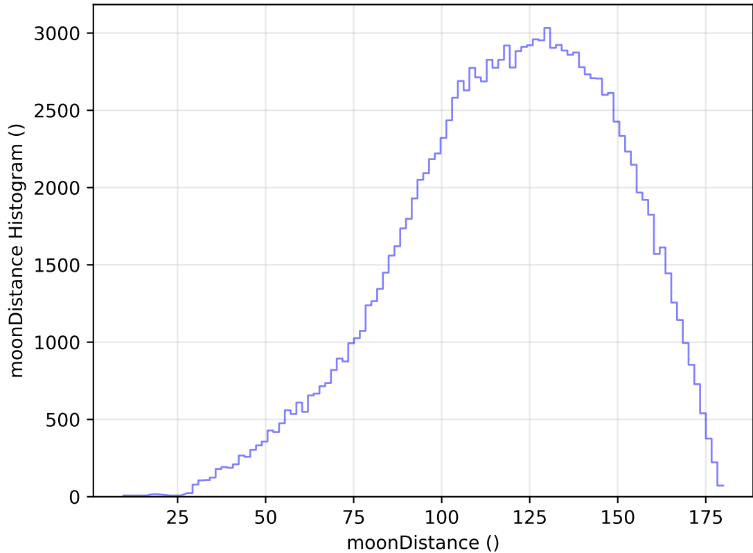
internal_u_expt38_nscale1.2v3.4_10yrs WFD u band: moonDistance Histogram
