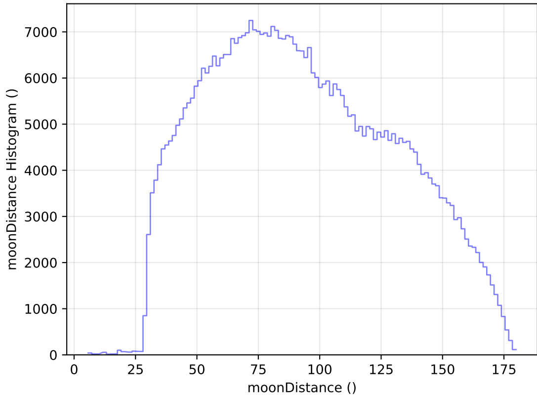
internal_u_expt38_nscale1.2v3.4_10yrs WFD i band: moonDistance Histogram
