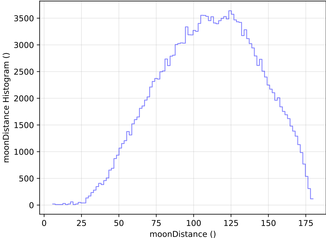
internal_u_expt38_nscale1.2v3.4_10yrs WFD g band: moonDistance Histogram
