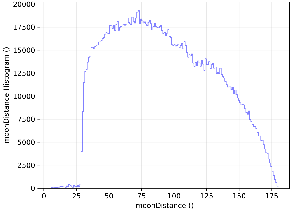
internal_u_expt38_nscale1.2v3.4_10yrs WFD all bands: moonDistance Histogram
