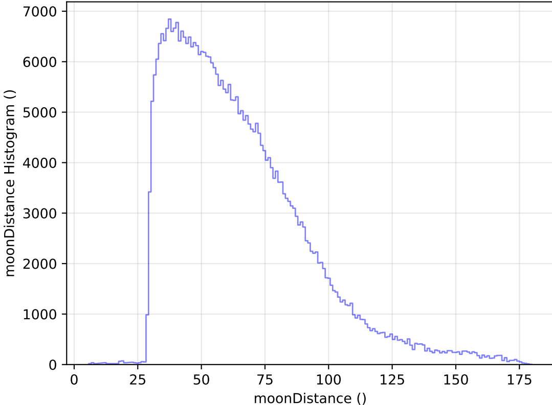
internal_u_expt38_nscale1.2v3.4_10yrs All sky y band: moonDistance Histogram
