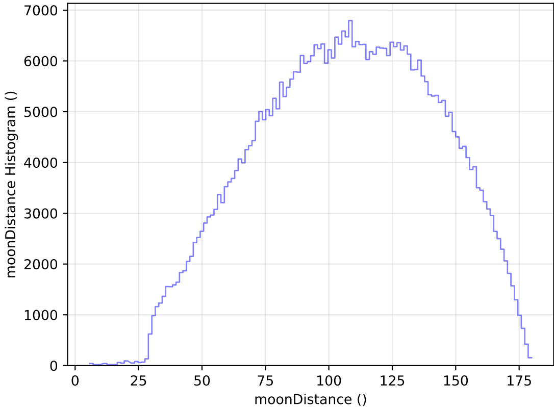
internal_u_expt38_nscale1.2v3.4_10yrs All sky r band: moonDistance Histogram
