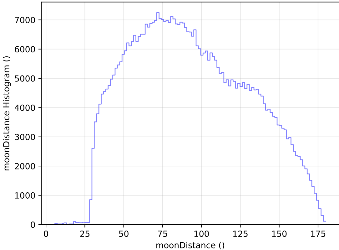
internal_u_expt38_nscale1.2v3.4_10yrs All sky i band: moonDistance Histogram
