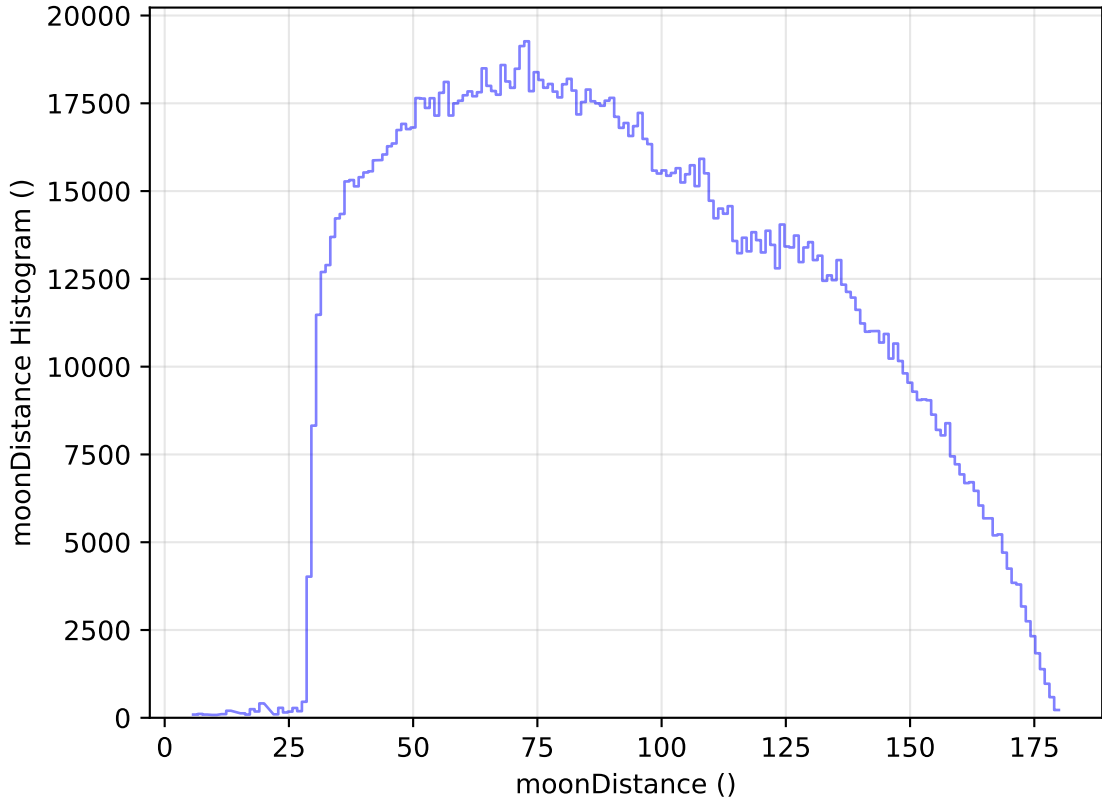
internal_u_expt38_nscale1.2v3.4_10yrs All sky all bands: moonDistance Histogram
