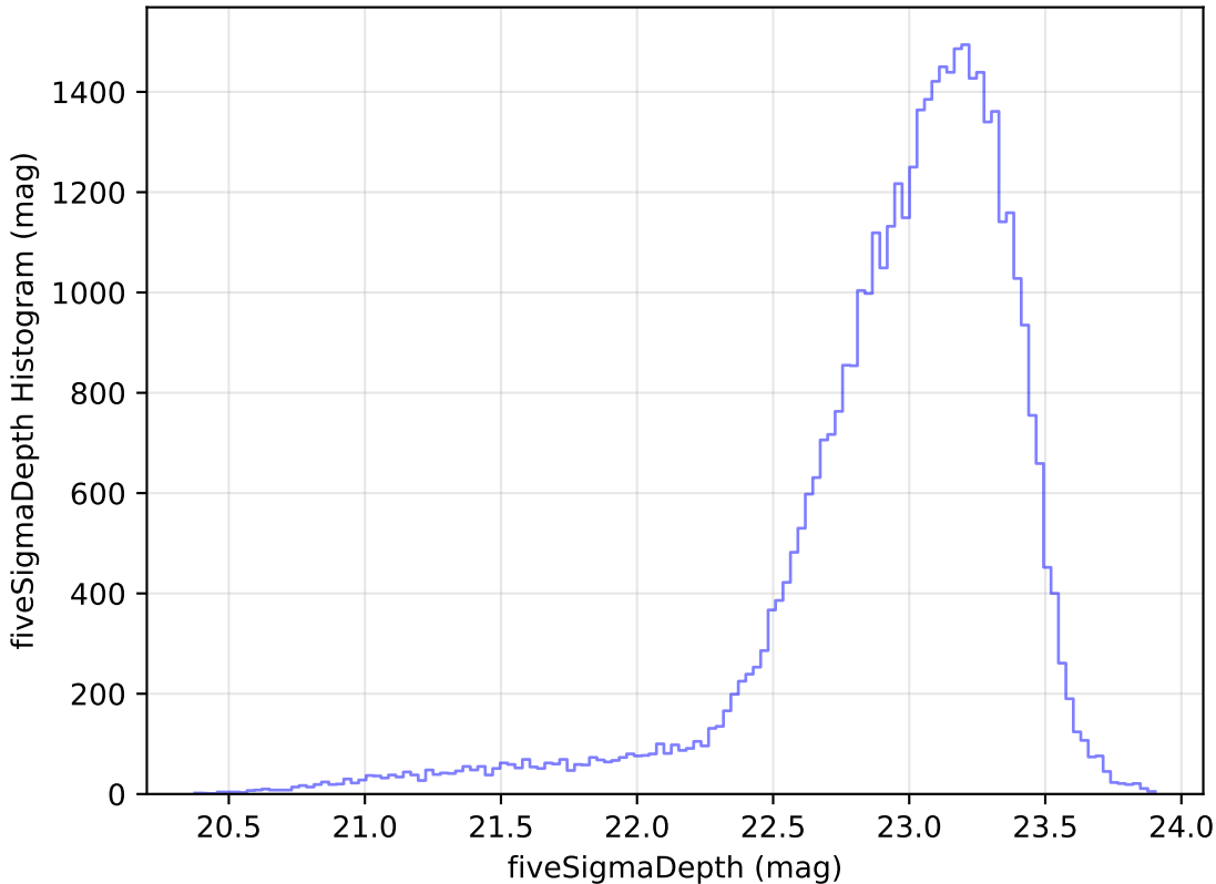
internal_u_expt38_nscale1.2v3.4_10yrs Yr 1 z band: fiveSigmaDepth Histogram
