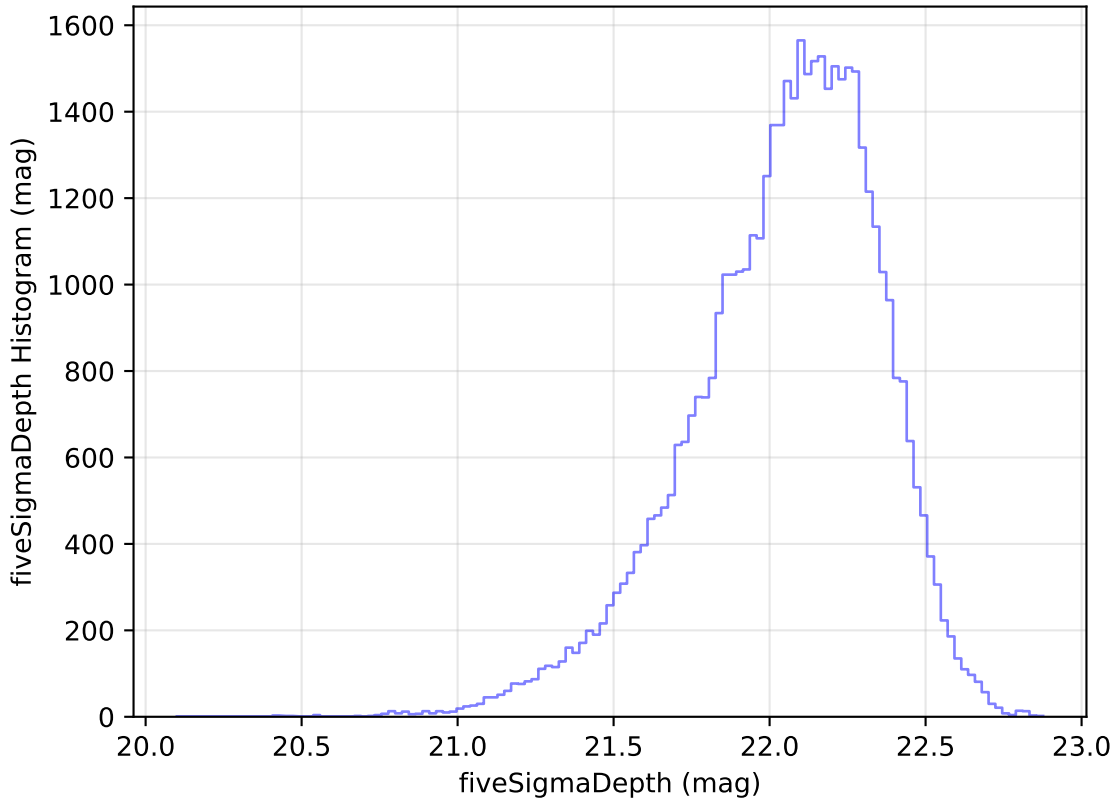
internal_u_expt38_nscale1.2v3.4_10yrs Yr 1 y band: fiveSigmaDepth Histogram
