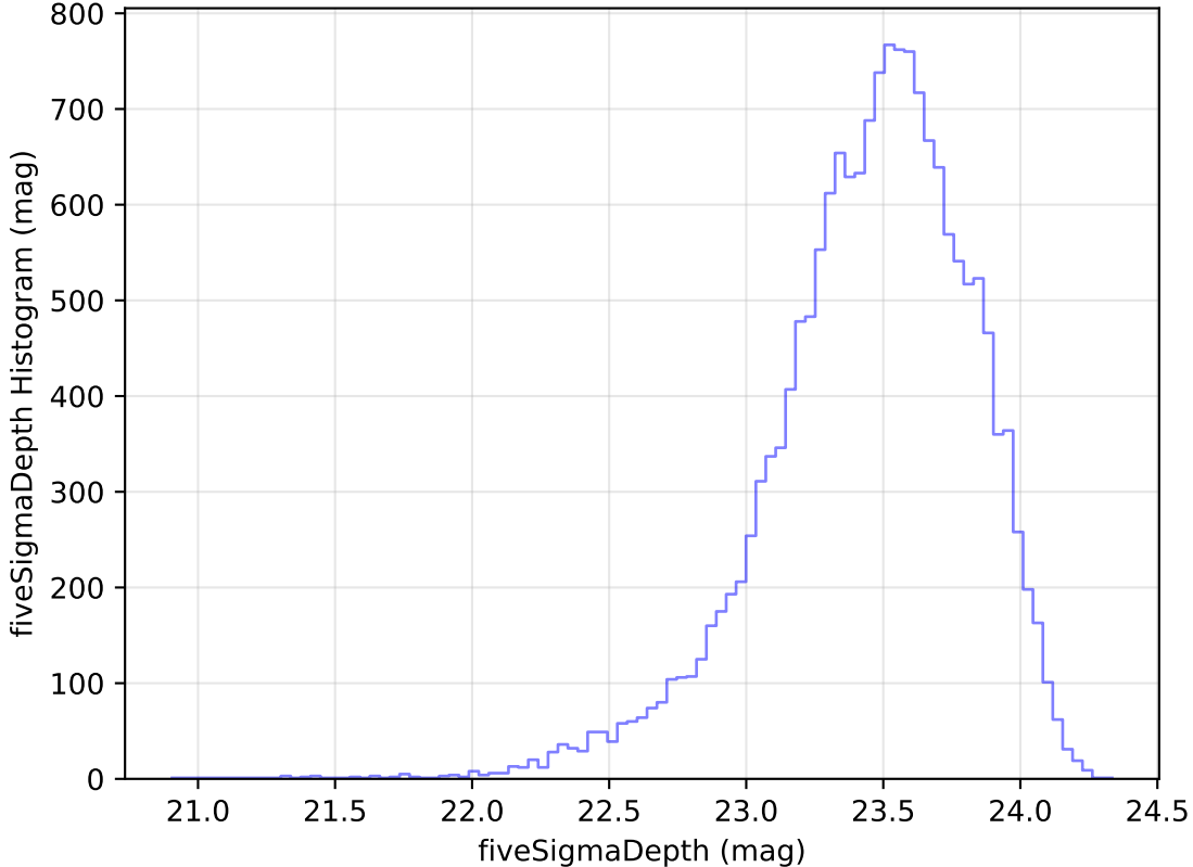
internal_u_expt38_nscale1.2v3.4_10yrs Yr 1 u band: fiveSigmaDepth Histogram
